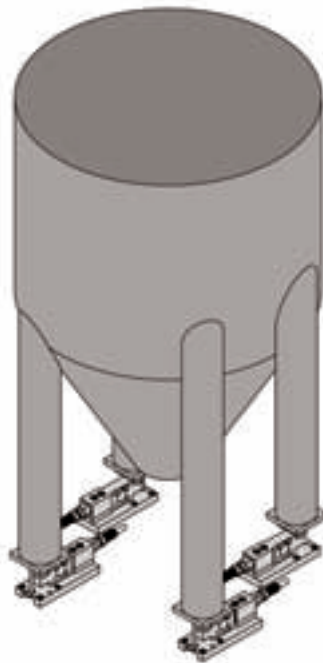
(Left to right) These illustrations show a vessel with compression load cells and another with tension load cells.
